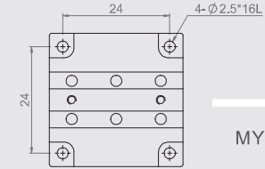
MX(Y)30-A-18 Mounting Dimensions
