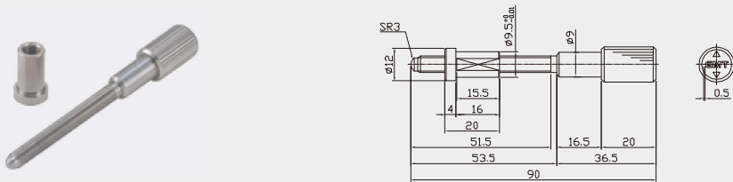
Model No : PS1R □—25 ; Threaded Screw : M6x [Pitch : 0.5 or 1]
