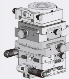
Micro-alignment module for AOI system.
