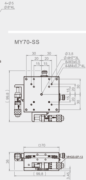
MX(Y)70-S Mounting Dimensions
