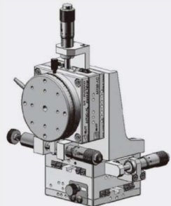
Micro-alignment module of CCD fabricated equipment.
