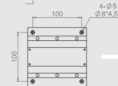
MX(Y)120-A-18 Mounting Dimensions
