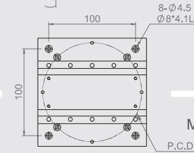
MX(Y)L125-A Mounting Dimensions
