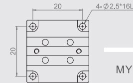
MX(Y)25-A-18 Mounting Dimensions
