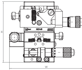
Front side viewing
