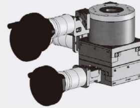
XYR-axis alignment stage module.
