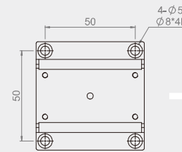
MX(Y)60-S-28 Mounting Dimensions
