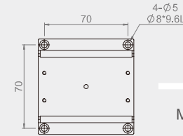
MX(Y)80-S-28 Mounting Dimensions
