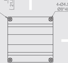
MX(Y)L90-A Mounting Dimensions
