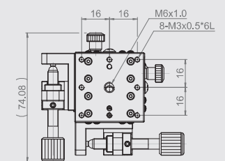
MX(Y)40-A-18 Mounting Dimensions
