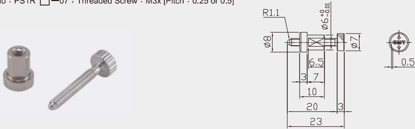
Model No : PS1R □—07 ; Threaded Screw : M3x [Pitch : 0.25 or 0.5]
