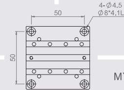
MX(Y)L60-A Mounting Dimensions
