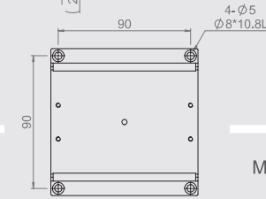
MX(Y)100-S Mounting Dimensions
