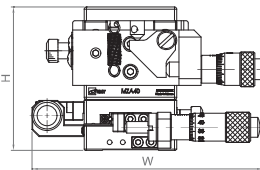
Front side viewing
