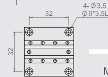
MX(Y)40-A-18 Mounting Dimensions
