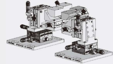
LED wafer characteristic inspection stage module.
