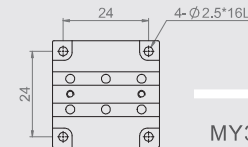
MX(Y)30-A Mounting Dimensions
