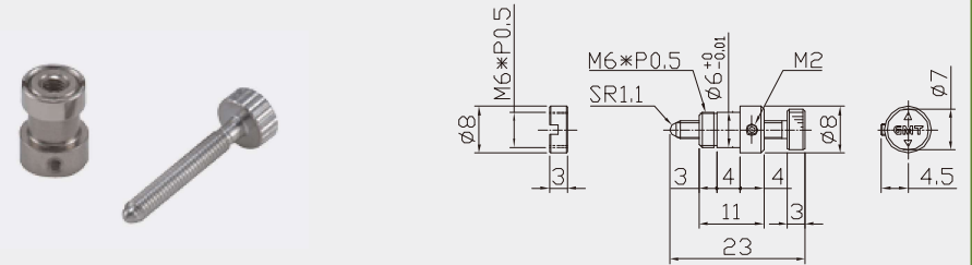
Model No : PS1M □—07 ; Threaded Screw : M3x [Pitch : 0.25 or 0.5]
