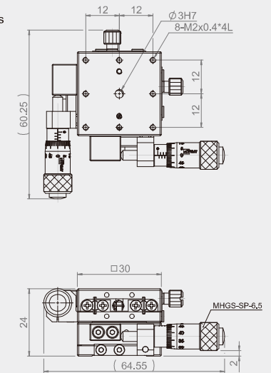
MX(Y)30-S Mounting Dimensions
