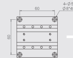
MX(Y)70-A Mounting Dimensions
