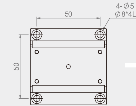
MX(Y)60-S Mounting Dimensions
