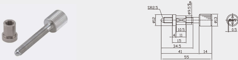
Model No : PS1R □—13 ; Threaded Screw : M6x [Pitch : 0.25 or 0.5]
