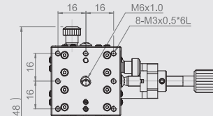
MX(Y)40-A-18 Mounting Dimensions
