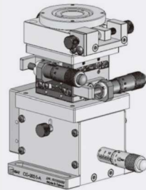
Micro-alignment module for AOI system.
