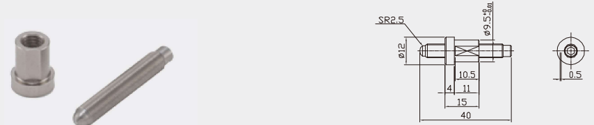
Model No : PS2R □—13 ; Threaded Screw : M6x [Pitch : 0.25 Or 0.5]
