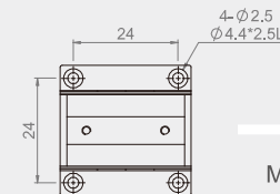
MX(Y)30-S Mounting Dimensions
