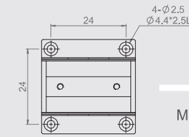
MX(Y)30-S-28 Mounting Dimensions
