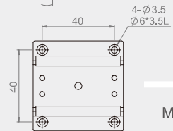
MX(Y)50-S Mounting Dimensions
