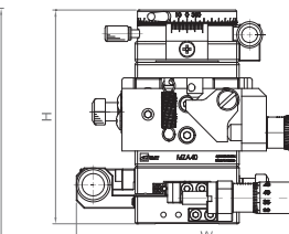
Front side viewing
