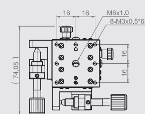
MX(Y)40-A-18 Mounting Dimensions
