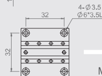
MX(Y)40-A-18 Mounting Dimensions
