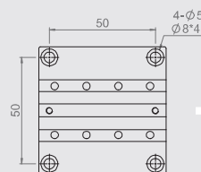
MX(Y)60-A-18 Mounting Dimensions
