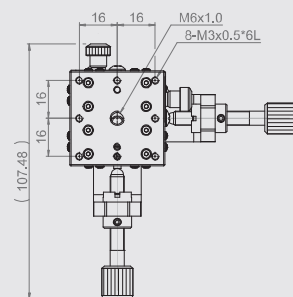
MX(Y)40-A-18 Mounting Dimensions
