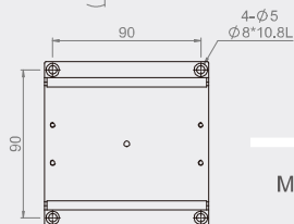
MX(Y)100-S-28 Mounting Dimensions
