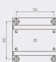
MX(Y)60-S-28 Mounting Dimensions
