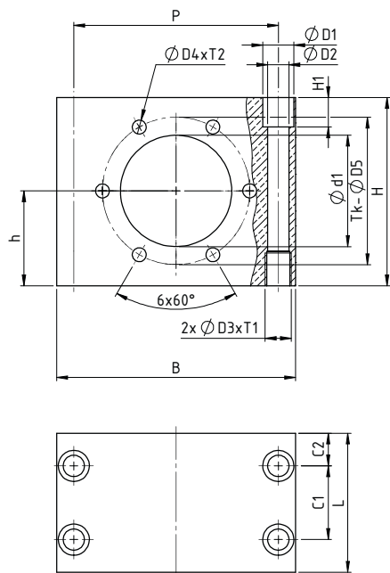
Bohrbild 3 passend zu TGM-EFM/KGF-N
