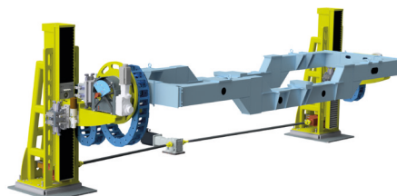
Lift and rotate unit
