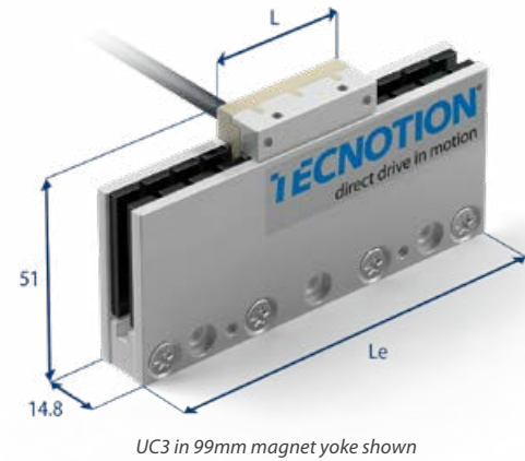
UC3 in 99mm magnet yoke shown
