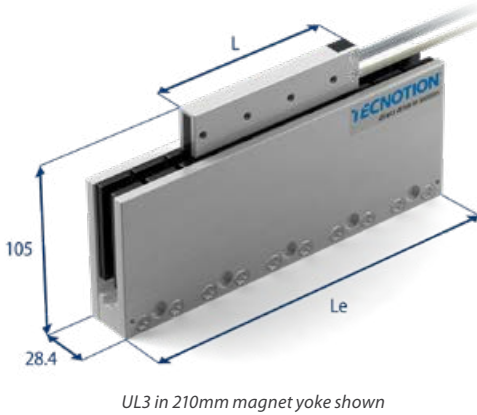
UL3 in 210mm magnet yoke shown
