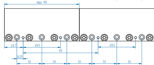
2x UC 99mm
