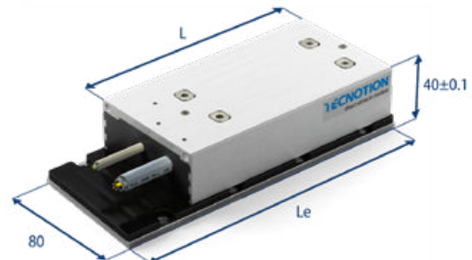
TL6 on 192mm magnet plate shown
